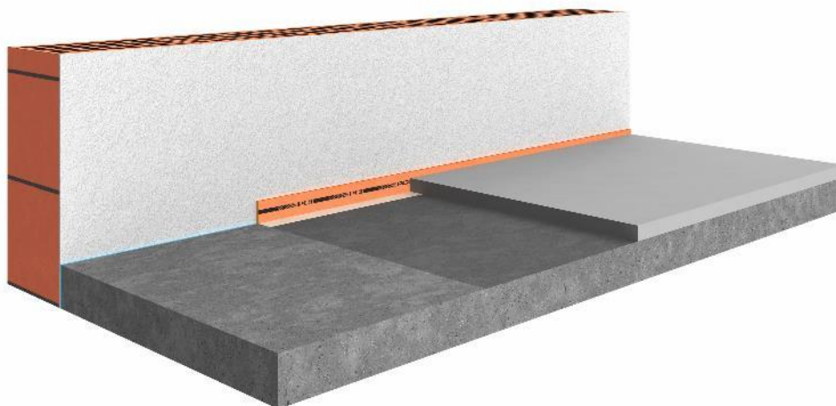
PCI system solution for fast screed repair ( Link to high-resolution photo )
